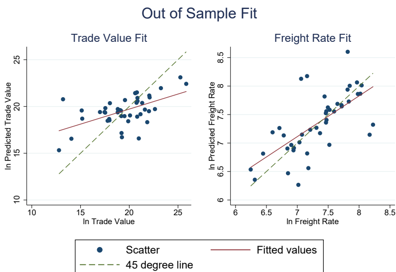
Figure A.5: Out of Sample Fit
