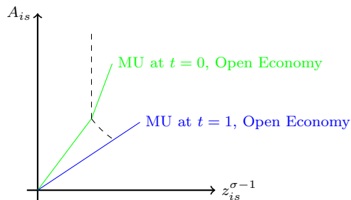
Figure M.2: Set of unconstrained and marginally constrained firms in open economy at t = 0, 1 .
