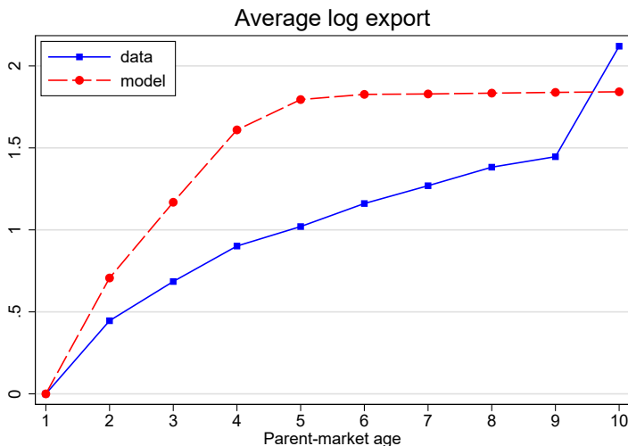
Figure 3: Export-age profile: data v.s. model
