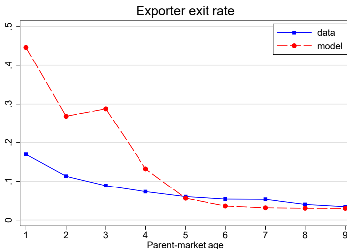
Figure 4: Exit rate - age profile: data v.s. model
