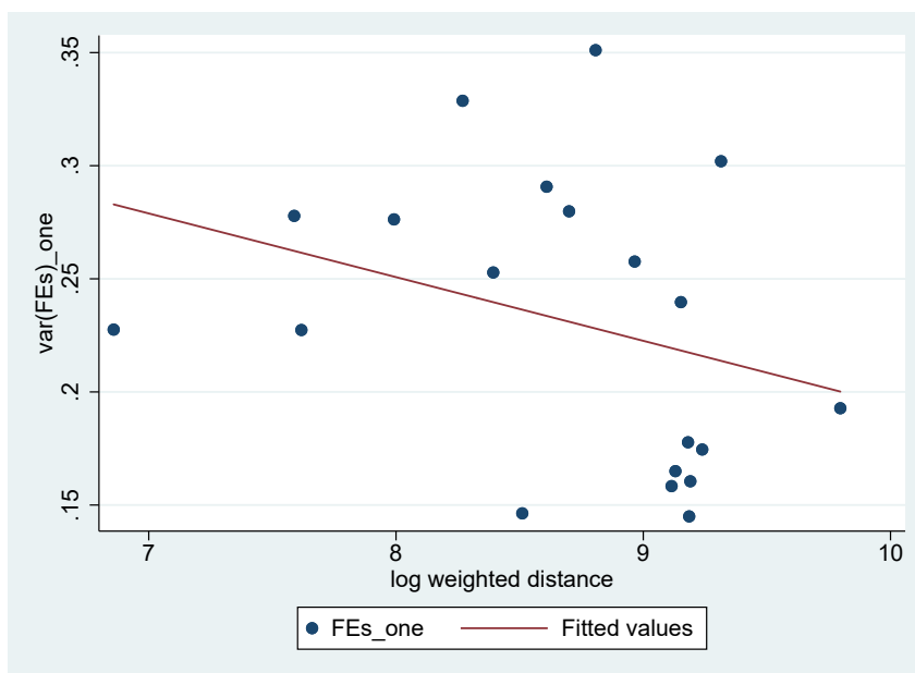
Figure 7: Initial Uncertainty (age-one) and Distance
