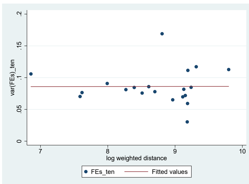
Figure 8: Eventual Uncertainty (age-ten or above) and Distance
