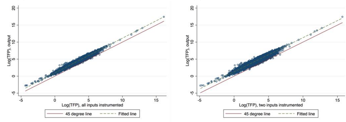
Figure A.11: The correlation between OLS and IV generated TFP, output method (a) All inputs instrumented with lags (b) Two inputs instrumented with lags
