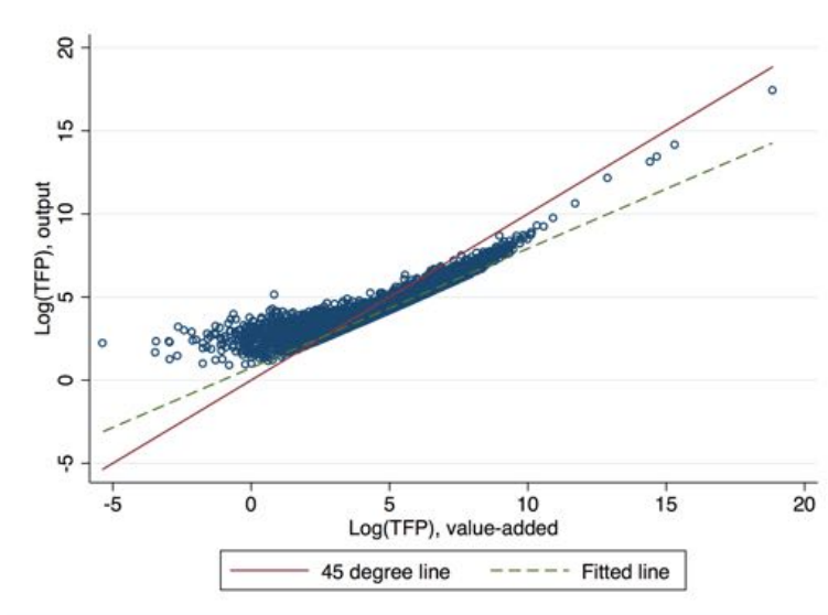
Figure A.10: The relationship between the TFP from the output method and value-added method, OLS
